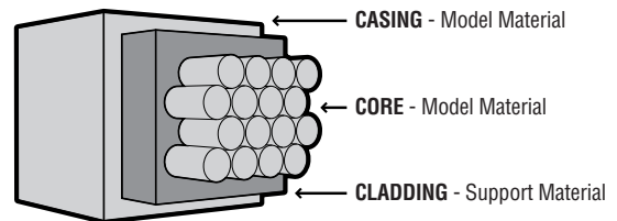
Figure 6: Light pipes consist of a rigid transparent core, a soft cladding, and a rigid outer casing.
